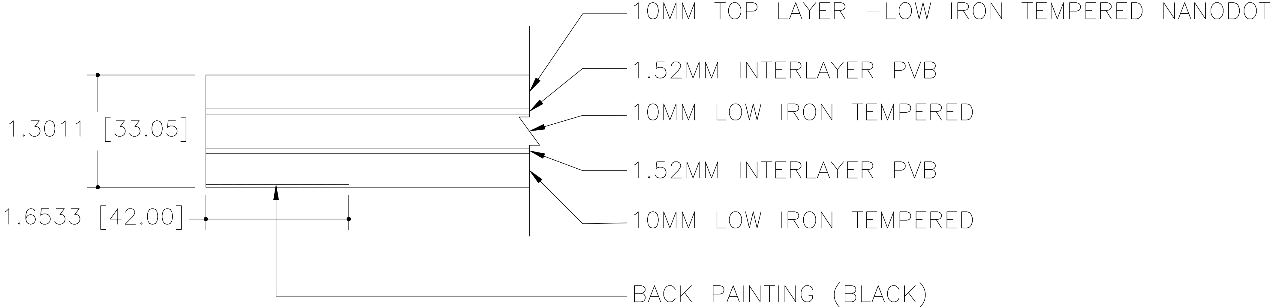
1 DETAIL - PERIMETER GLASS ASSEMBLY
