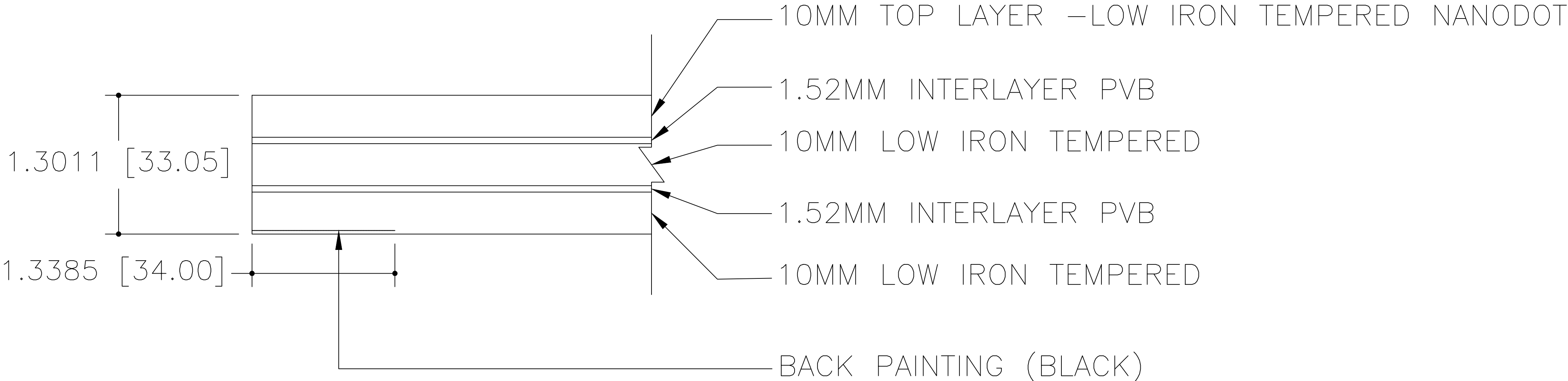
2 DETAIL - RAFTER GLASS ASSEMBLY
